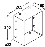
Recessing box
