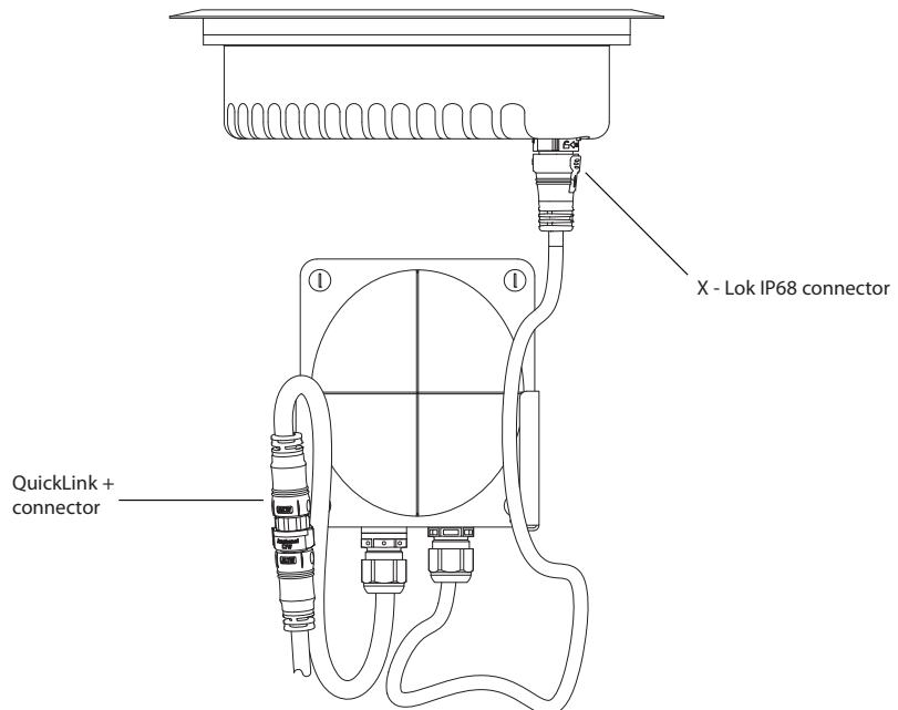
Luminaire & driver
