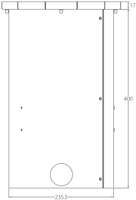
Ground Mount Front & Rear view
